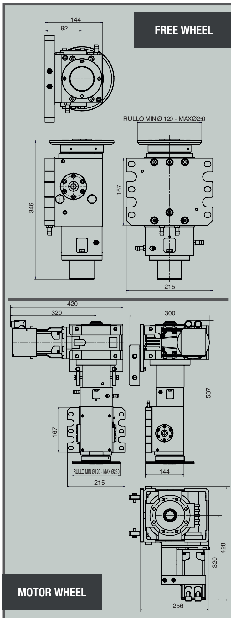
WATER-COOLED SEAM WELDING HEADS
