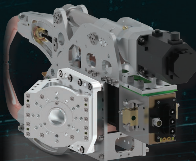
45° connection every guns is available in its right or left mirror configuration and symmetrical guns
