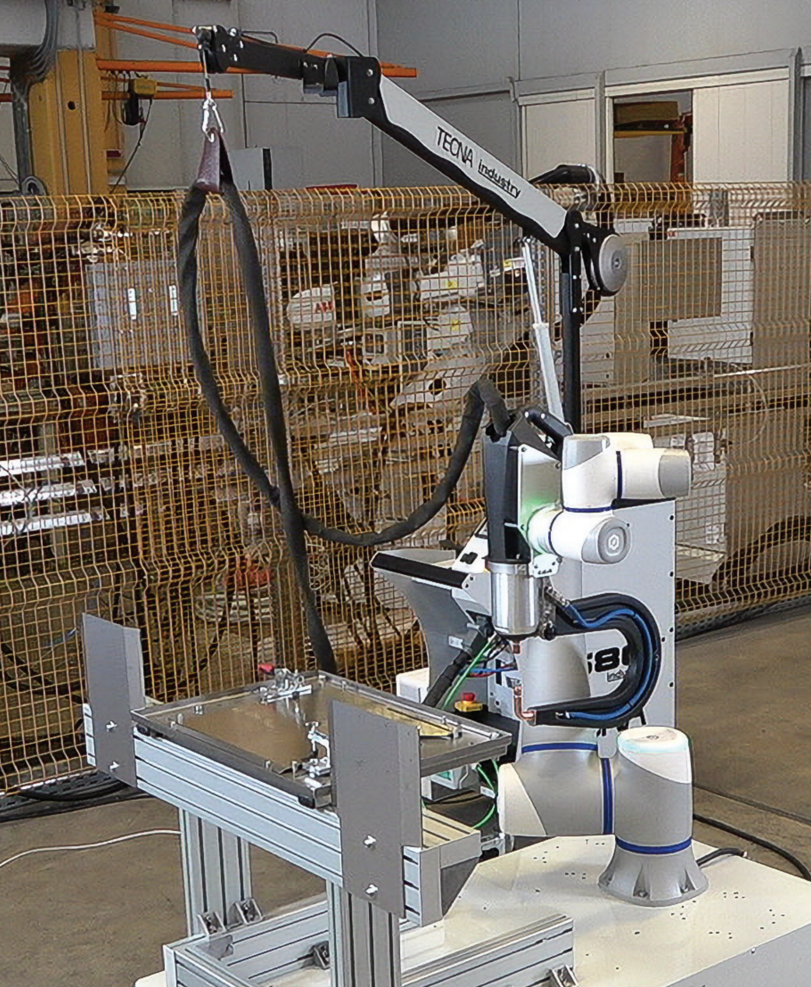
3680S Industry pneumatic spot welding station
